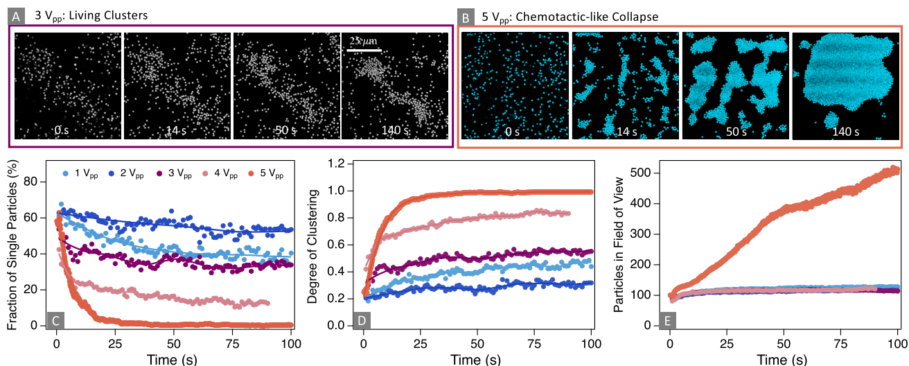
Fig. 4. Versatile nonequilibrium aggregation: from living clusters to chemotactic collapse. Sequence of images for 1.75 μm CB-PS particles, and 100 Hz: (A) at 3 V_{pp} demonstrating transient aggregation, and (B) at 5 V_{pp} demonstrating rapid coarsening. Characteristic horizontal black-cyan shades at 140 s correspond to waves on the assembled 2D micro sheet, with a wavelength around \lambda \approx 25 μm. These waves represent slight variations in the vertical focusing position of particles. (C) Fraction of single particles defined as the number of single particles relative to the total number of particles in the field of view at a given time. (D) Degree of clustering, as introduced in Ref. [46], \theta(t) = 1 - 1/\langle n_{\text{clust}}(t) \rangle where \langle n_{\text{clust}}(t) \rangle is the mean cluster size at a given time. (E) Total number of particles in the field of view, rescaled by the number of particles in the field of view at the beginning of image acquisition. In (C-E), cluster properties are measured with increasing V_{pp} , at 100 Hz, with the legend shared across plots. Dots are data points and lines are guides for the eye corresponding to window averages. These experiments were performed with 1.75 μm CB-PS particles, with concentration of approximately 5 \times 10^{-2}\% w/v, and an average \zeta = -65.0 \pm 3.1 mV. For clarity, fluorescence images for 3 and 5 V_{pp} are reported in grayscale and false colors, respectively.
