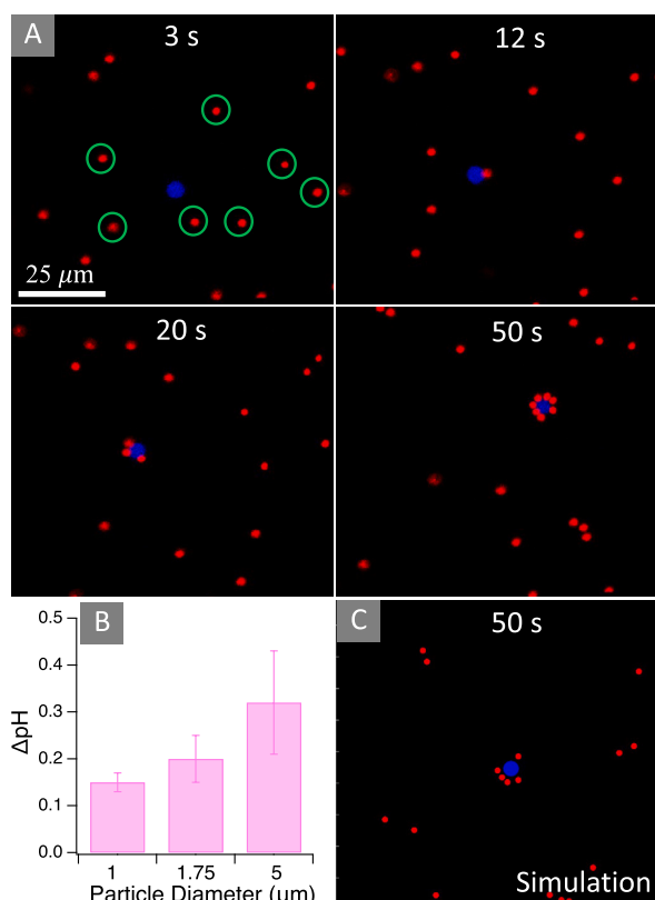
Fig. 5. Interparticle potential mediates capture of smaller particles. (A) Sequence of images for 5 μm (blue) surrounded by 2 μm (red) CB-PS particles at the levitated layer under 5 V pp and 100 Hz. A large particle behaves as a beacon for smaller particles, indicated by green circles. (B) Size dependence of ΔpH. Error bars in Panel B represent the standard deviation of values from ten frames and ten different particles, for a total of 100 points. (C) Characteristic result of a Brownian dynamics simulation with interparticle potentials fitted from experimental data and initial configurations from (Panel A, 3s). The simulation domain is a square, with sides equal to 115 μm.
